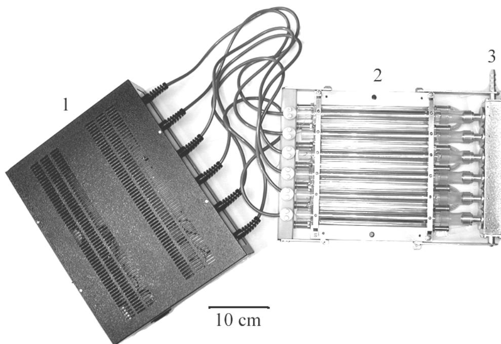
General view of BD_Cs line excilamps: 1 – power supply; 2 – six bulb's cascade; 3 – cooling system.
